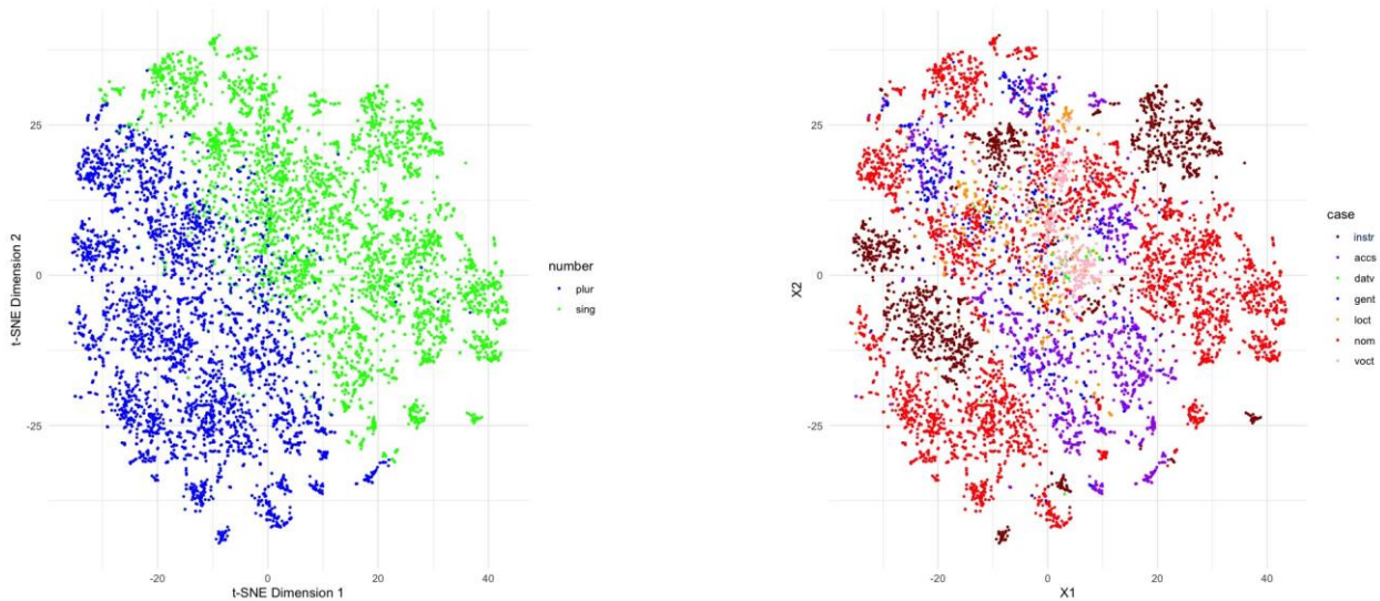
Figure 2: Distribution of Ukrainian non-syncretic nouns restricted to those with both singular and plural forms in the dataset, without case restrictions. The left panel demonstrates a clear, binary bifurcation of the vector space, confirming that grammatical number is the dominant organizing principle for Ukrainian nouns. In contrast, the right panel reveals significant intra-cluster diffusion among grammatical cases. The lack of distinct case boundaries—even in this filtered, non-syncretic dataset—empirically illustrates that case alternations (such as the Accusative-Genitive overlap) are deeply embedded in the distribution of the language, whereas the distinction between singular and plural remains a robust, primary structural divide
