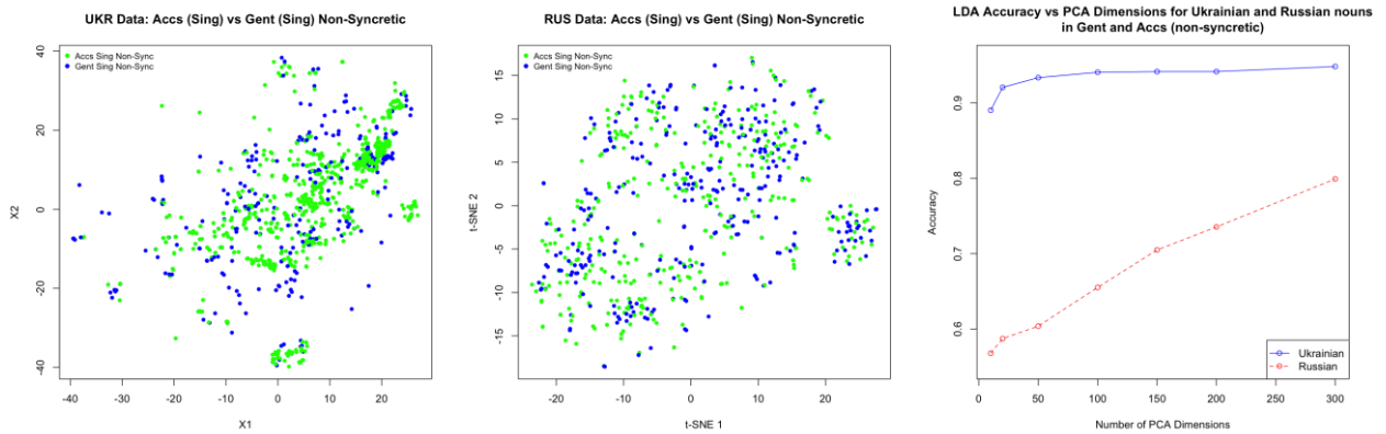
Figure 5: Distribution of Ukrainian and Russian non-syncretic translation equivalents of singular nouns in Genitive (in blue) and Accusative (in green). Left panel: Ukrainian, center panel: Russian, right panel: LDA classification accuracies for increasing numbers of principal components of the embedding spaces
