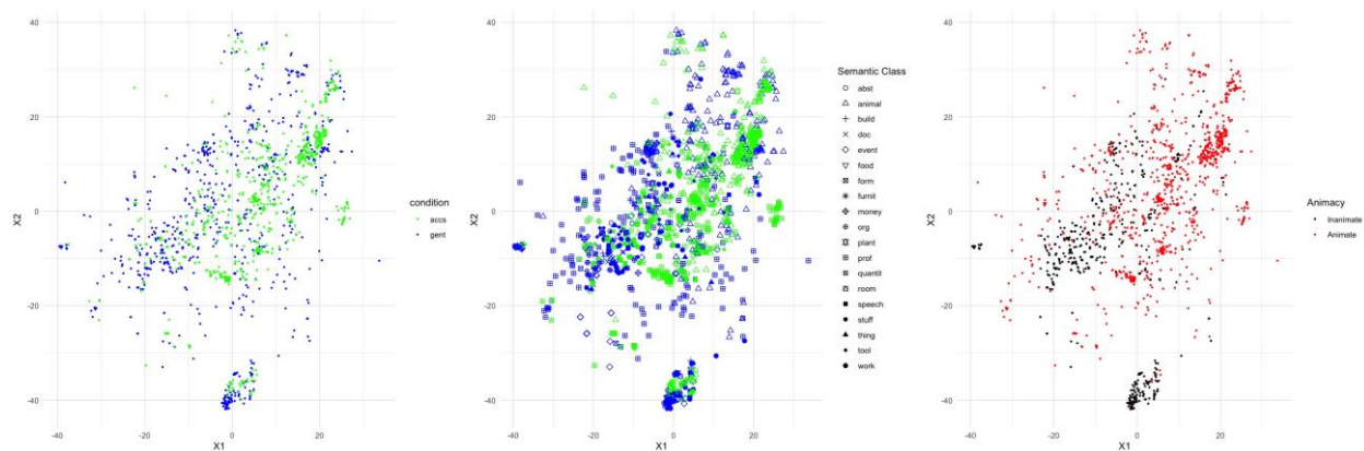
Figure 4: Distribution of Ukrainian nouns in Genitive (in blue) and Accusative (in green) cases. The left plot illustrates the distribution of Ukrainian nouns in genitive and accusative cases. The middle plot presents their distribution in Genitive and Accusative cases within semantic classes. The right panel highlights the distribution of animate and inanimate nouns within genitive and accusative cases
