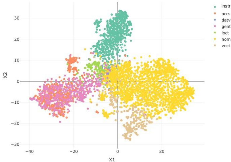
Figure 3: Distribution of Ukrainian shift vectors for number shows considerable clustering by case
