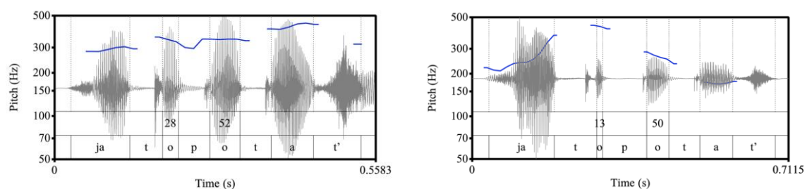
Fig. 1. Start of the utterance ' Ja topotát' uže ne búdu ', in two different renditions by speaker M11F from Moscow, in Praat (Boersma & Weenink 1992-2026), showing oscillogram, F0 curve (blue line) and durations of the pretonic vowels in ms.
