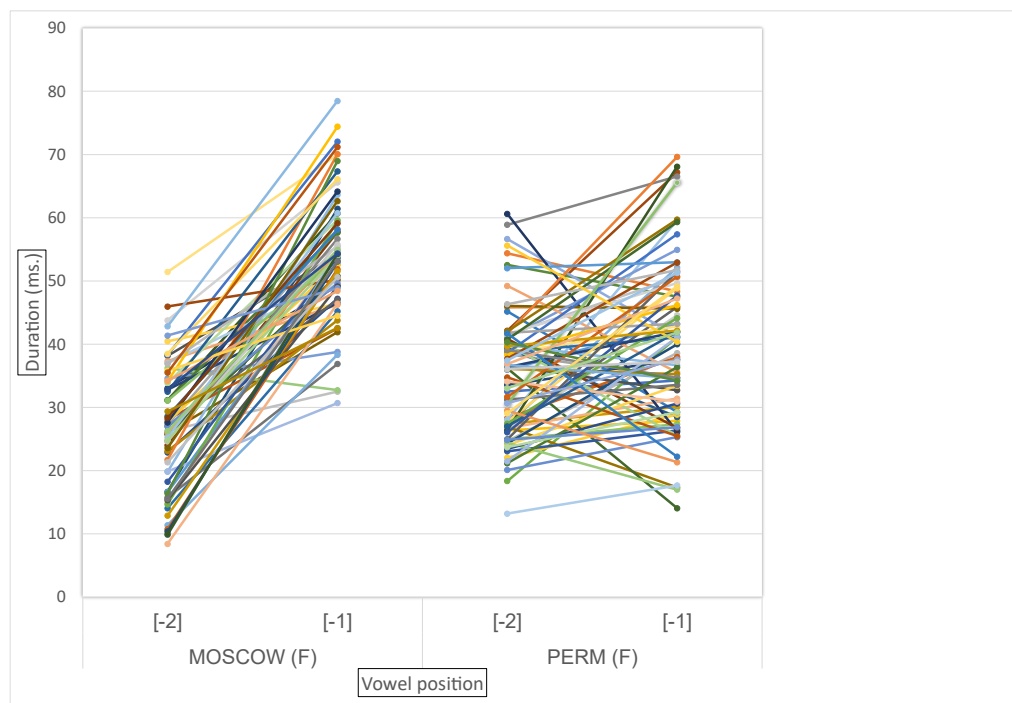
Fig. 2. Durations (in ms.) of the second ( a_{-2} ) and first pretonic vowels ( a_{-1} ) in all individual word tokens of topotát' , pokopát' and potakát' by the female speakers in Moscow (left) and Perm (right).
