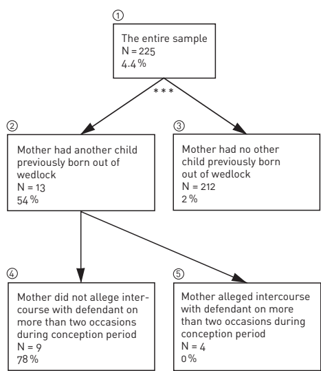
DIAGRAM A. AID analysis of the old sample, the results of the paternity suits functioning as dependent variable (successful claim = 0, dismissed claim = 1).
