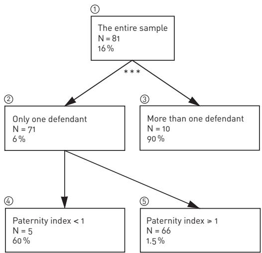
DIAGRAM B. AID analysis of the new sample, the results of the paternity suits functioning as dependent variable (successful claim = 0, dismissed claim = 1).
